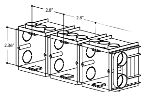
horizontal installation
