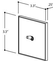
SINGLE FRAME
