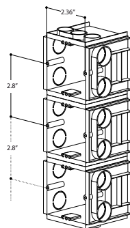
vertical installation
